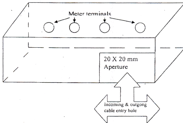
Terminal cover of Single phase Fully Static meter
