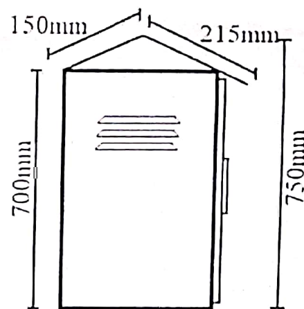
300mm SIDE VIEW
