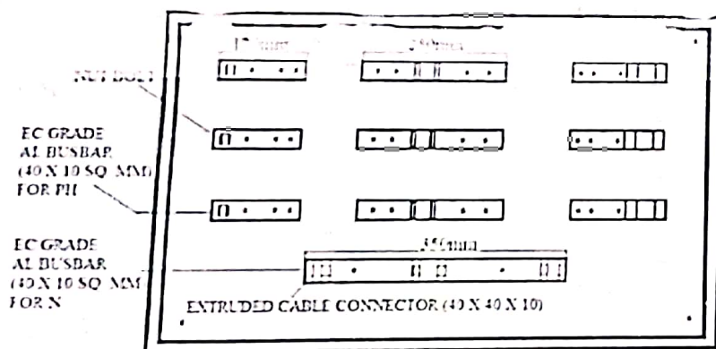
FRONT VIEW WITHOUT DOOR
