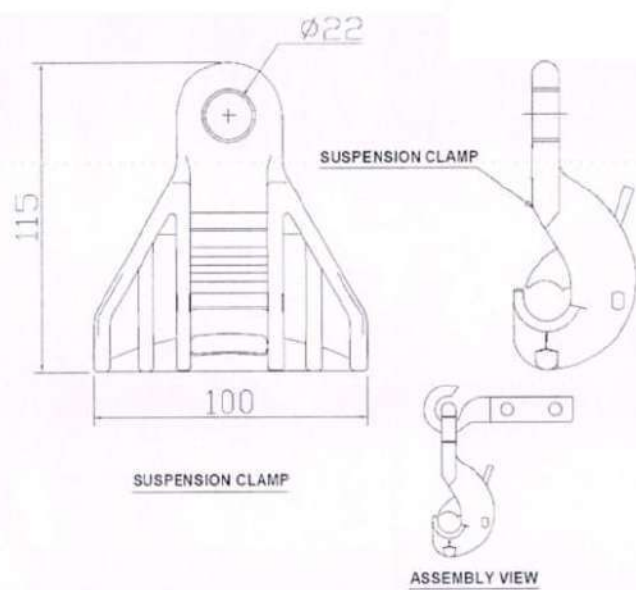
Suspension Clamp Eye Hook Type Suitable For 25-95 Sq.mm. Bare/Insulated Messenger Wire
