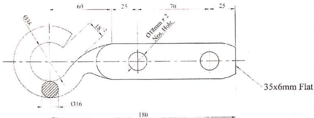
Eye Hook (Type 'A' for use with Pole Clamp)
