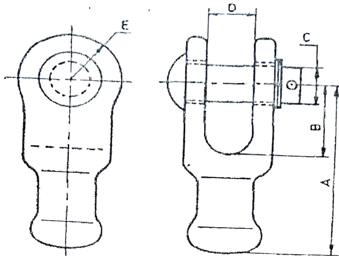
Fig 2: Ball Clevis
