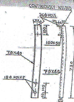
FIG-2 TOP ADAPTER
