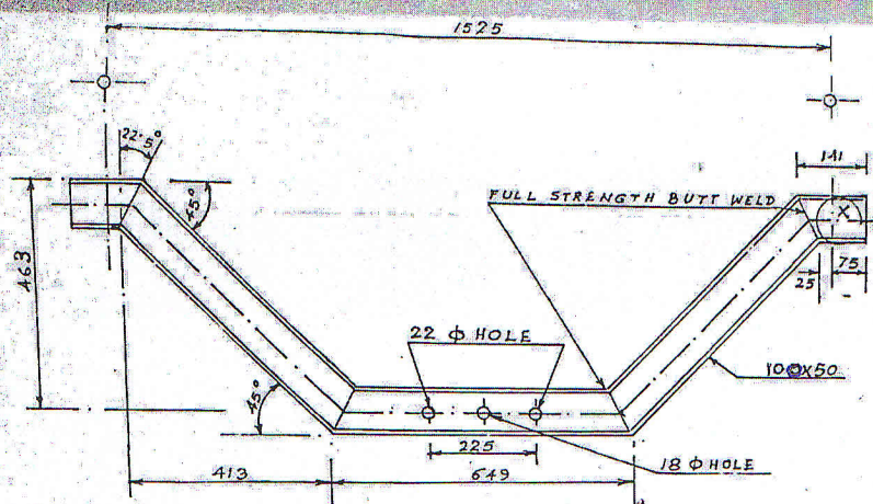
FIG-1 V-BRACKET
