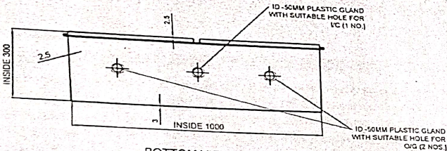
BOTTOM VIEW
