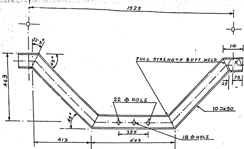
FIG-1 V-BRACKET
