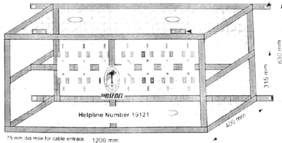
Front view with cover
