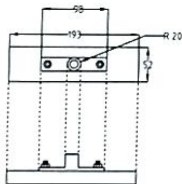
HANDLE BASE TOP & FRONT VIEW
