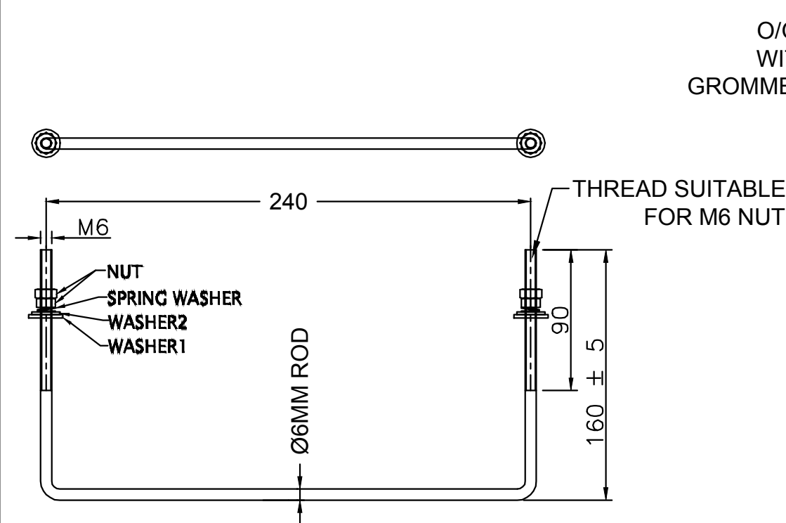
MS POLE MOUNTING CLAMP - 2NOS./BOX
