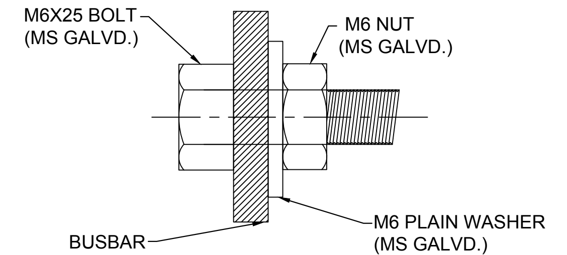
CONNECTION BOLT
