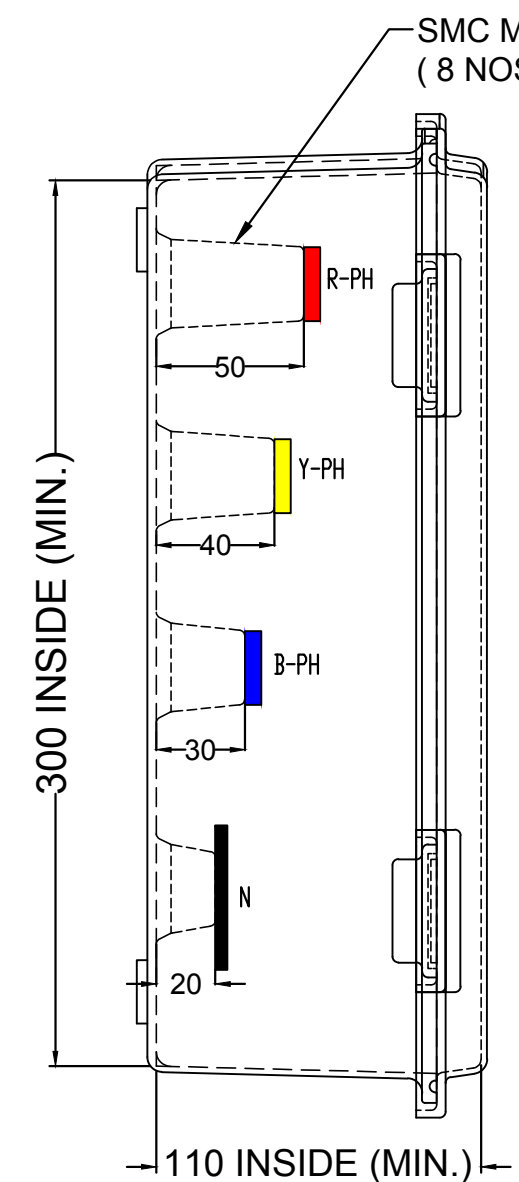
SIDE CLEAR VIEW
