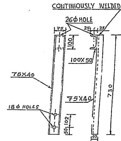
FIG-2 TOP ADAPTER
