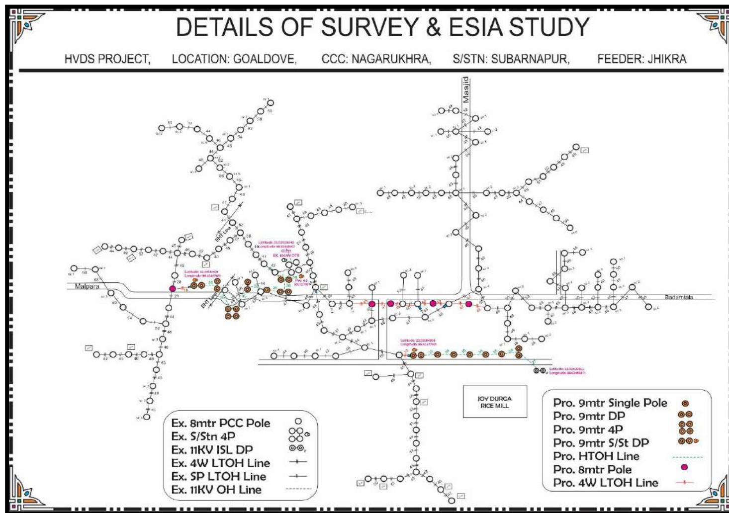
FIGURE 5.5: VIEW OF EXISTING HT/LT NETWORK OF SELECTED LOAD CENTRES FOR HVDS SUB-PROJECT AT NADIA DISTRICT (AT GOALDOVE 100 KVA DTR UNDER JHIKRA FEEDER)
